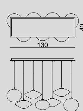
1679MX.40X130.7L SOSPENSIONE A PIASTRA / HANGING LAMP WITH CEILING PLATE Glass 7 x Ø 30-30-35 cm - Cable 200 cm 7 x LED 8,4 W DIMM
