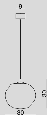
GIG1643.1L SOSPENSIONE A ROSONE / HANGING LAMP WITH CANOPY Glass 1 x Ø 30 cm - Cable 200 cm 1 x LED 8,4 W DIMM
